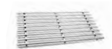
Multi-Chef™ Rectangle Stainless Steel Track Grill 23.25×11.75×0.75 in 59×305×2 cm Item # SM193
